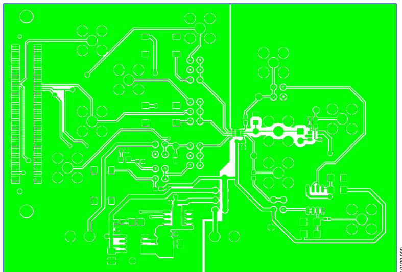
Figure 9. Component Side PCB Drawing
