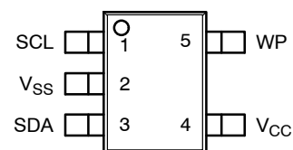
TSOT-23 (TD), TSOP-5** (TS) (Top View)
