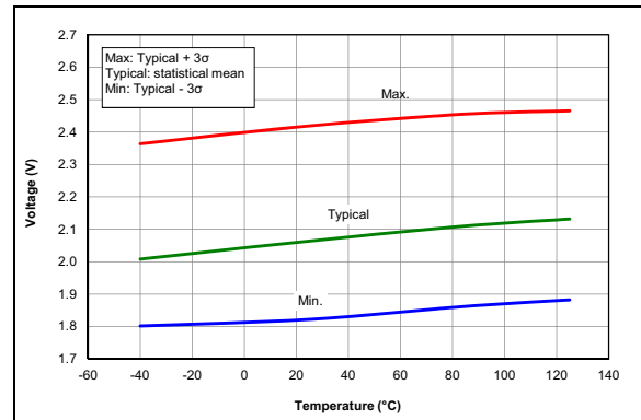
FIGURE 36-53: LPBOR Reset Voltage.
