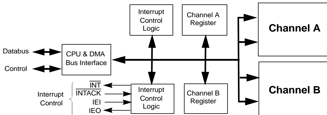
Figure 1.SCC Block Diagram
