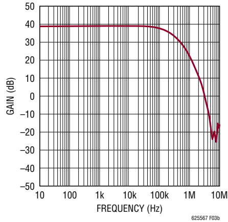
Figure 3. Gain of 100 Amplifier (3dB Bandwidth of 200kHz on 130μA Supply Current)
