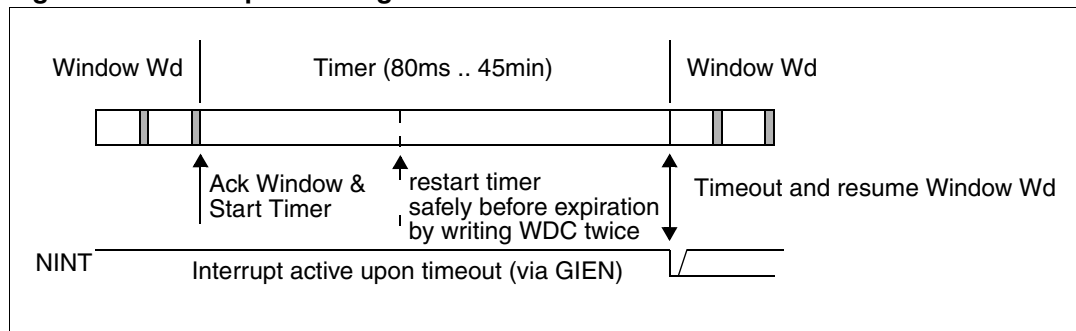
Figure 21. Wakeup watchdog
