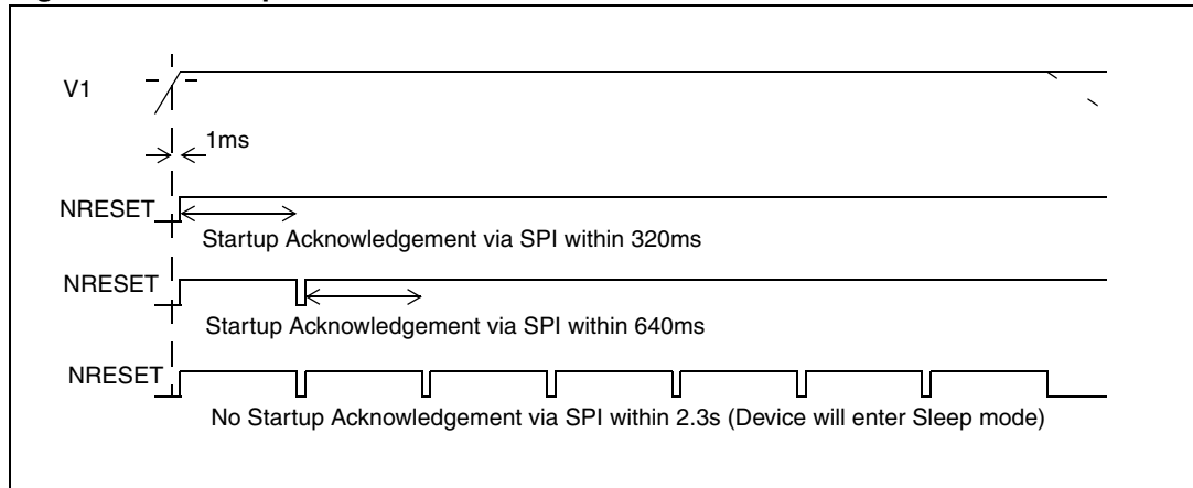
Figure 19. Startup
