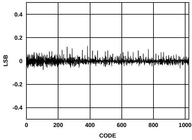
FIGURE 36. DIFFERENTIAL NONLINEARITY
