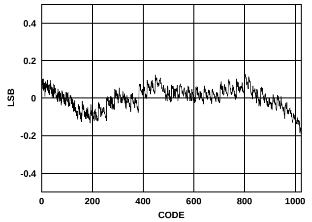
FIGURE 37. INTEGRAL NONLINEARITY
