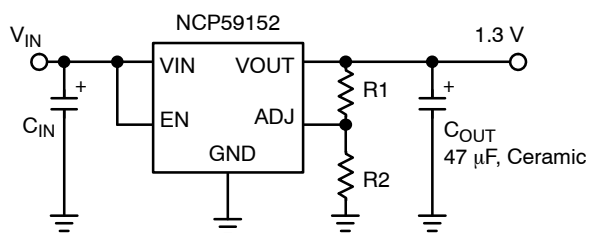
Figure 2. Adjustable Regulator
