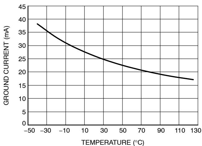
Figure 15. Ground Current vs. Temperature ( V_{OUTnom} = 2.5\text{ V} , I_{OUT} = 1.5\text{ A} , V_{IN} = 3.5\text{ V} )
