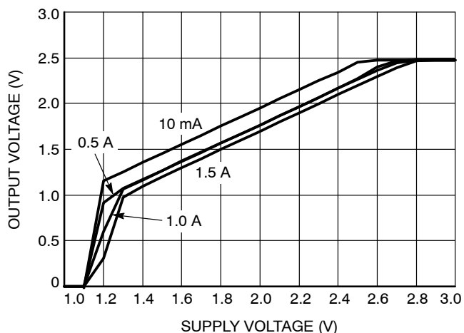
Figure 7. Dropout Characteristics ( V_{OUTnom} = 2.5\text{ V} )
