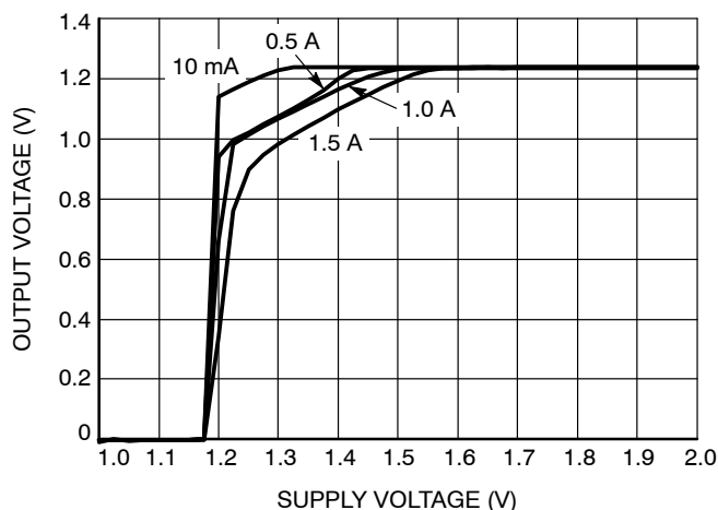
Figure 6. Dropout Characteristics ( V_{OUTnom} = 1.24\text{ V} )
