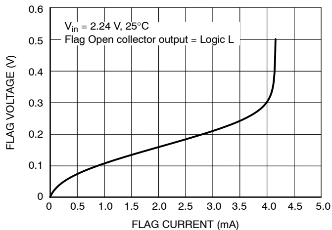
Figure 20. Flag Voltage vs. Flag Current
