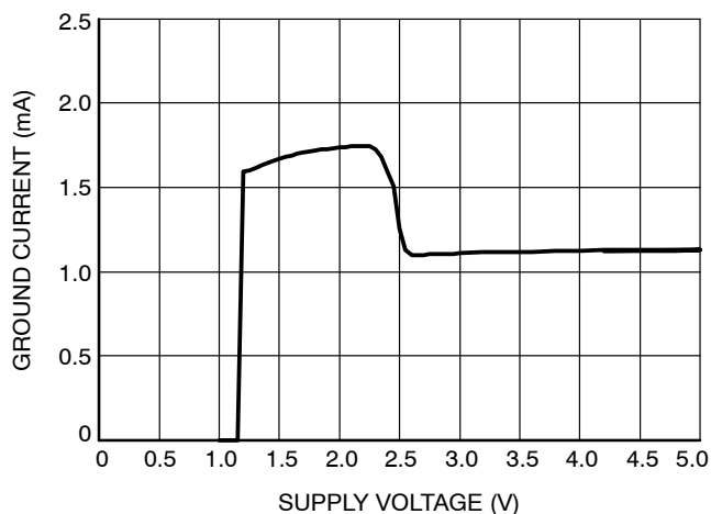
Figure 11. Ground Current vs. Supply Voltage ( V_{OUTnom} = 2.5\text{ V} , I_{OUT} = 10\text{ mA} )
