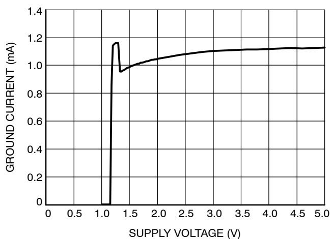
Figure 9. Ground Current vs. Supply Voltage ( V_{OUTnom} = 1.24\text{ V} , I_{OUT} = 10\text{ mA} )
