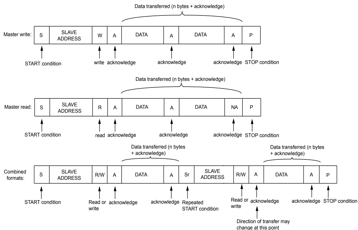
Figure 12. I²C data formats
