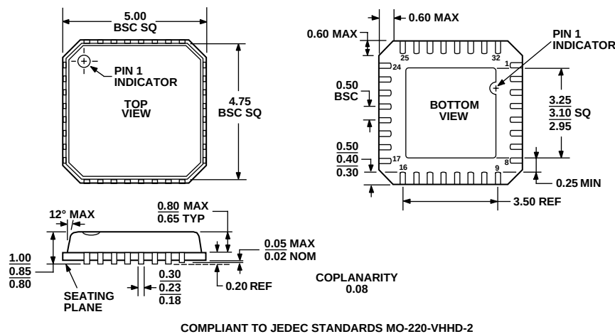
Figure 31. 32-Lead Frame Chip Scale Package [LFCSP] (CP-32) Dimensions shown in millimeters
