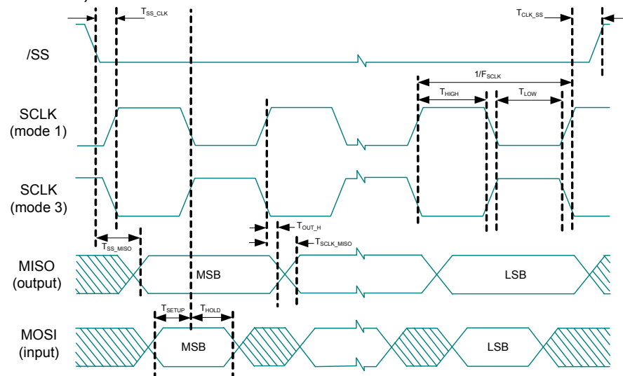
Figure 15. SPI Slave Mode 1 and 3
