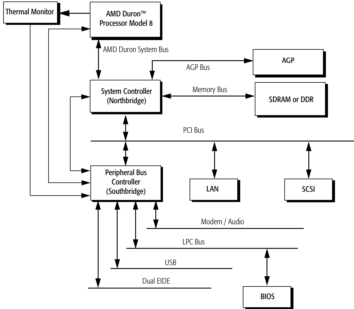
Figure 1. Typical AMD Duron™ Processor Model 8 System Block Diagram
