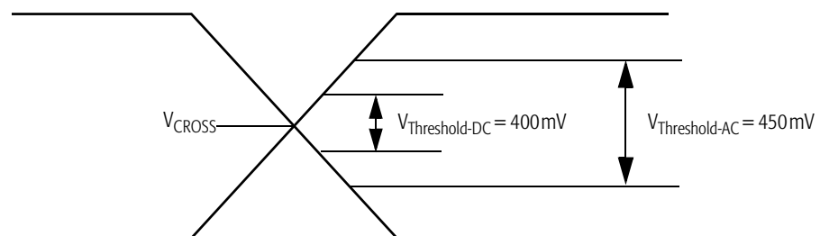
Figure 9. SYCLK and SYCLK# Differential Clock Signals
