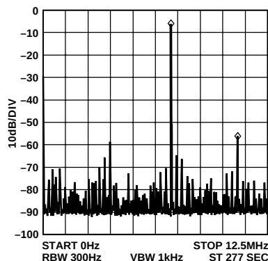
Figure 18. f_{MCLK} = 25 \text{ MHz} , f_{OUT} = 7.1 \text{ MHz} , Frequency Word = 48B43958
