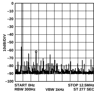
Figure 12. f_{MCLK} = 25 MHz, f_{OUT} = 1.1 MHz, Frequency Word = B439581
