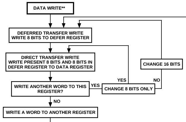
Figure 24. Data Writes
