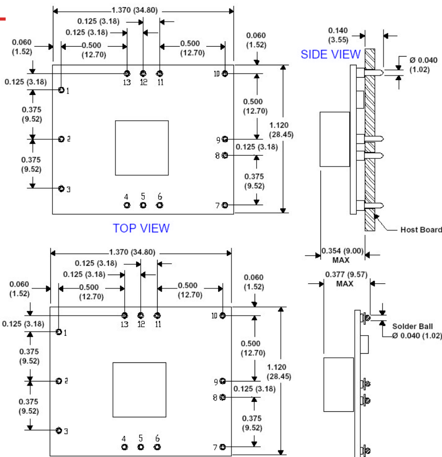
Through-hole and SMT Outline [in (mm)]
