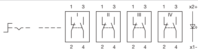
Wiring diagram 275
