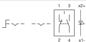
Wiring diagram 276
