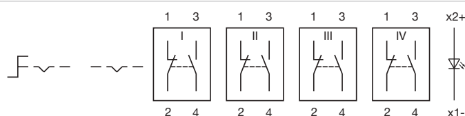
Wiring diagram 280
