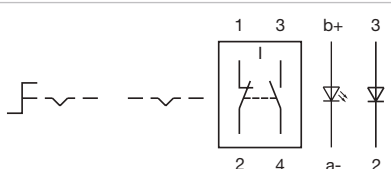
Wiring diagram 280
