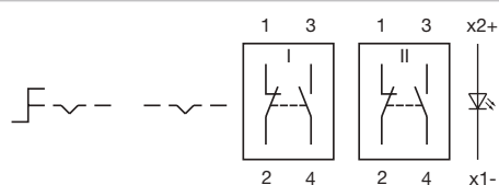
Wiring diagram 278
