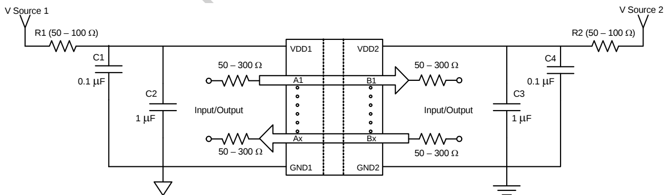
Figure 7. Recommended Bypass Components for the Si84xx Digital Isolator Family
