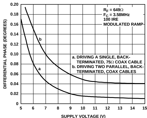
Figure 46. Differential Phase Error vs. Supply Voltage for the Video Line Driver of Figure 42
