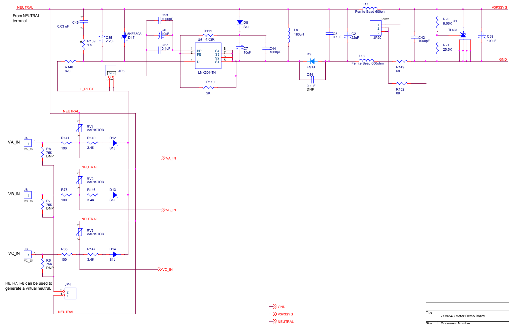
Figure 4-6: Teridian 71M6543 REV 5.0 Demo Board: Electrical Schematic 2/4
