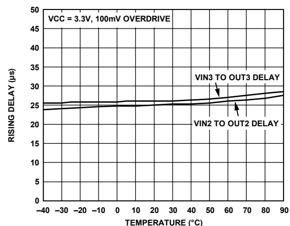
Figure 8. VIN2/VIN3 to OUT2/OUT3 Rising Delay vs. Temperature
