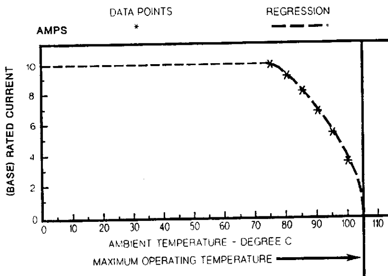
Figure 4A Current Carrying Capacity
