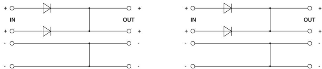
Block diagram
