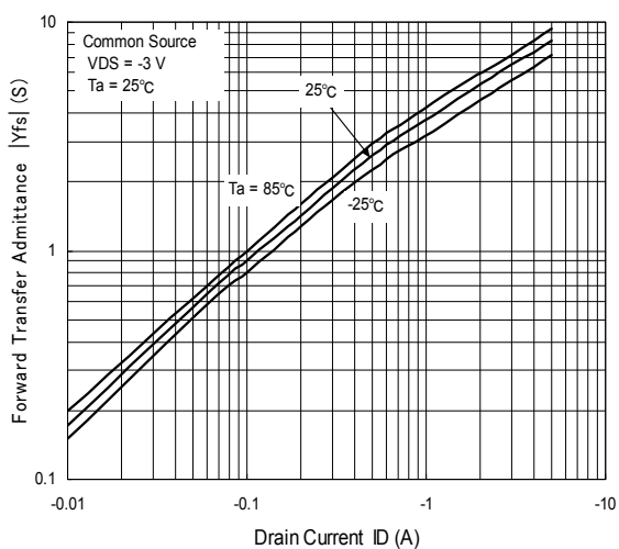
|Yfs| - VDS
