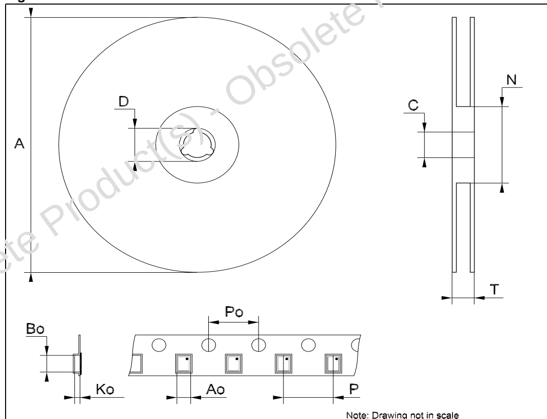
Figure 8. Reel dimensions
