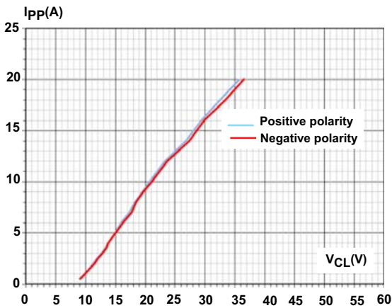
Figure 8. TLP measurements
