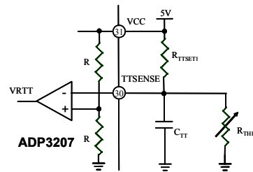
Figure 12. Single-Point Thermal Monitoring
