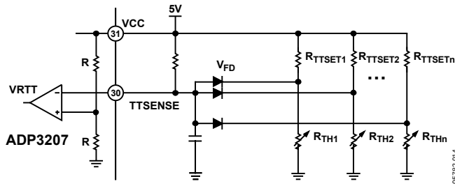
Figure 13. Multiple-Point Thermal Monitoring
