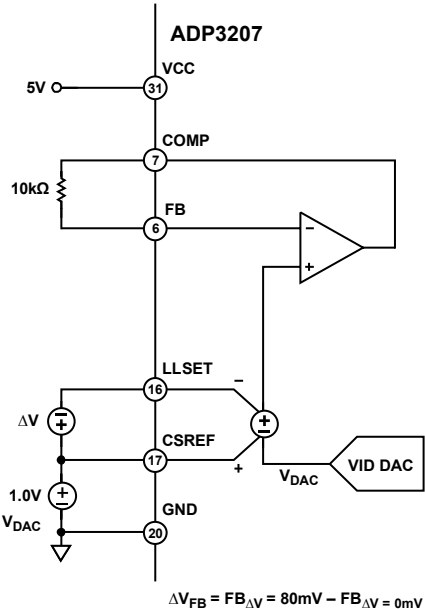
Figure 4. Positioning Accuracy
