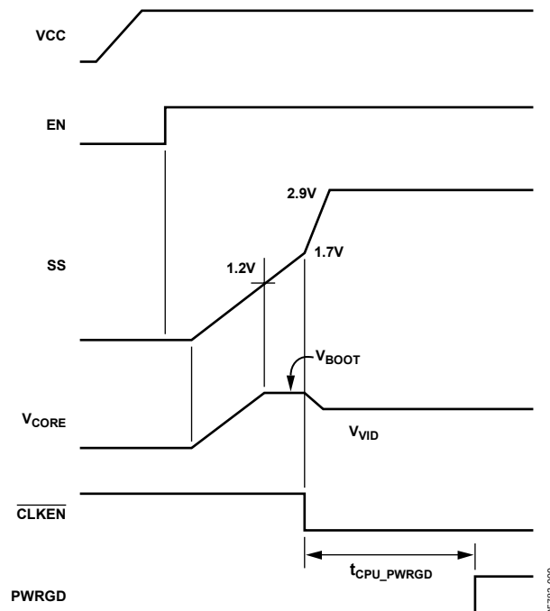
Figure 9. Power-Up Sequence
