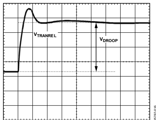
Figure 16. Transient Setting Waveform, Load Release
