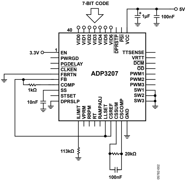
Figure 2. Closed-Loop Output Voltage Accuracy
