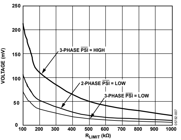
Figure 8. Current-Limit Threshold Voltage vs. R_{LIMIT}
