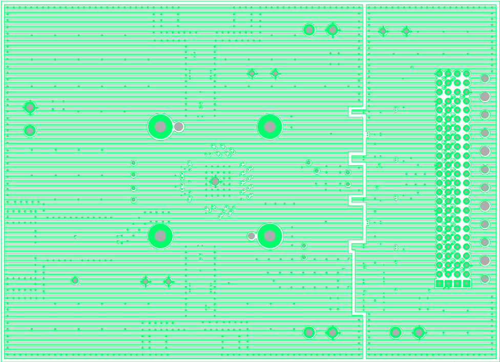
Layer 2: Ground
