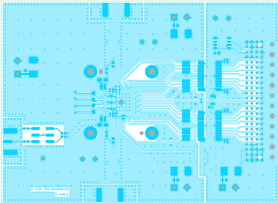
Layer 6: Circuit Side
