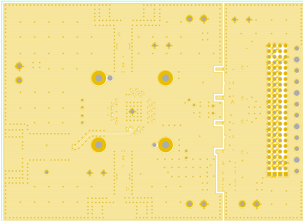
Layer 4: Ground, Clock
