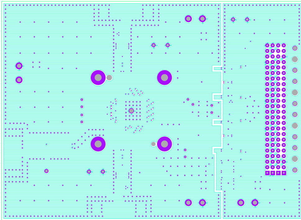
Layer 5: Ground
