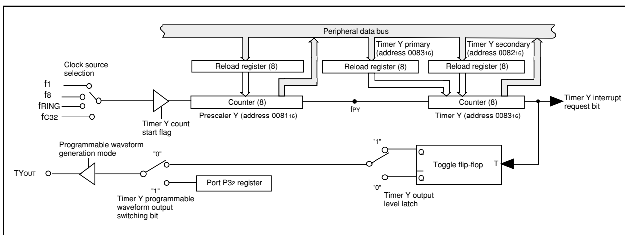
Figure 1.14.13. Block diagram of Timer Y
