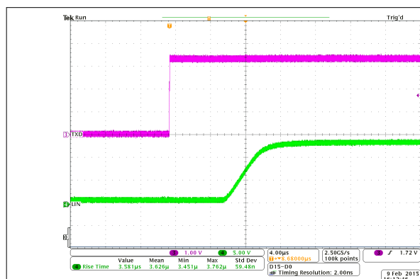
Figure 11-2. Dominant to Recessive Propagation Delay
