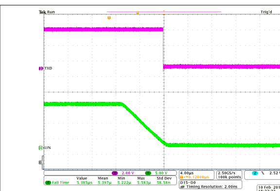
Figure 11-3. Recessive to Dominant Propagation Delay
