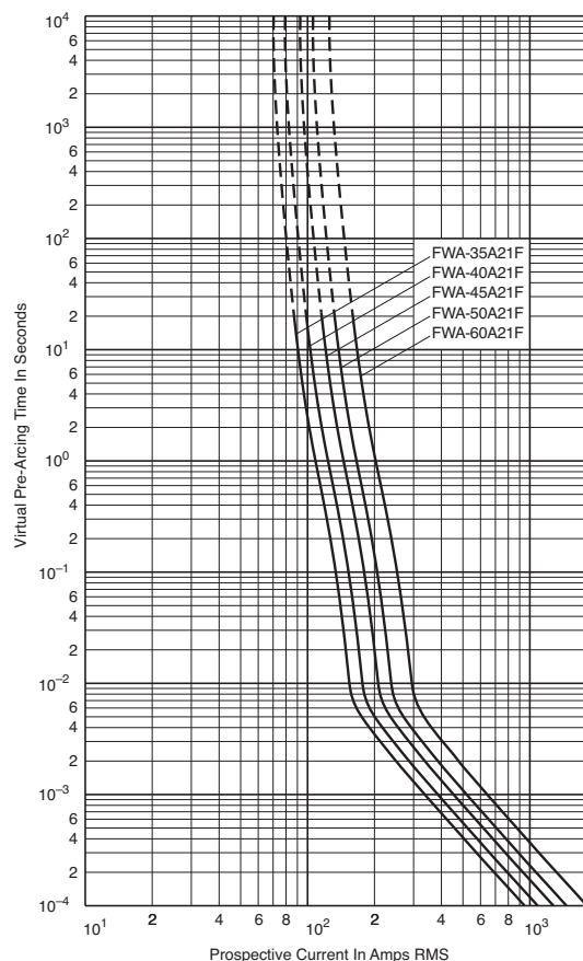
Time-Current Curve
