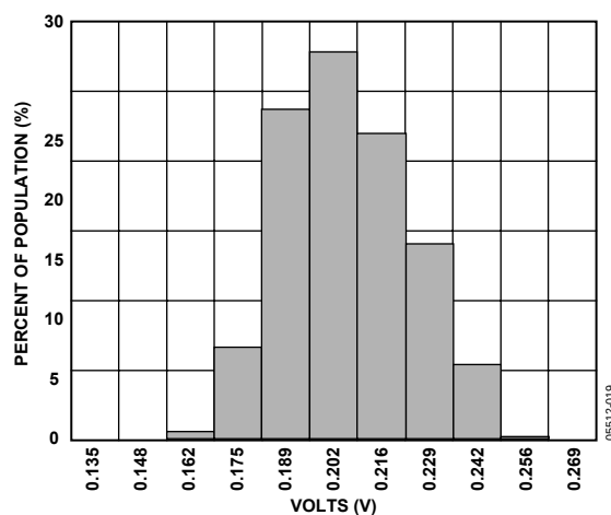
Figure 20. Y-Axis Self-Test Response at 25°C
