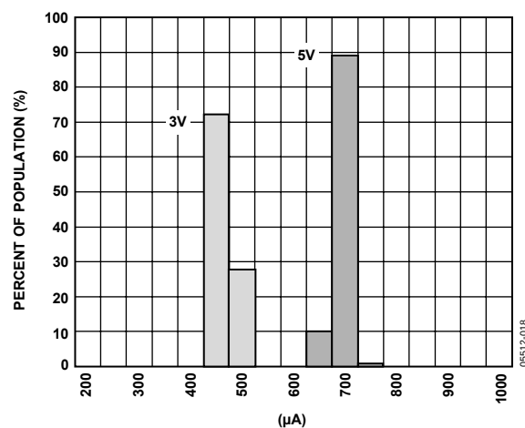
Figure 19. Supply Current at 25°C
