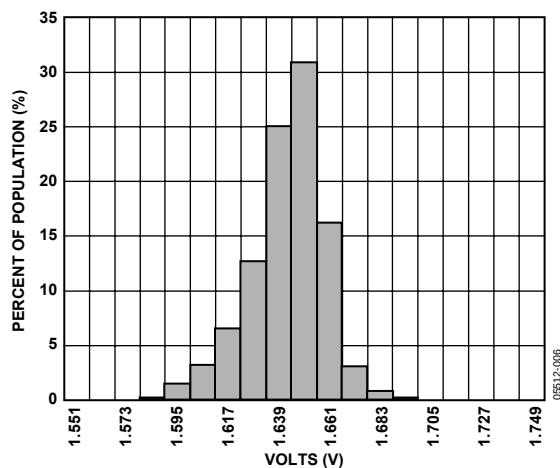
Figure 7. Y-Axis Zero g Bias Output at 25°C
