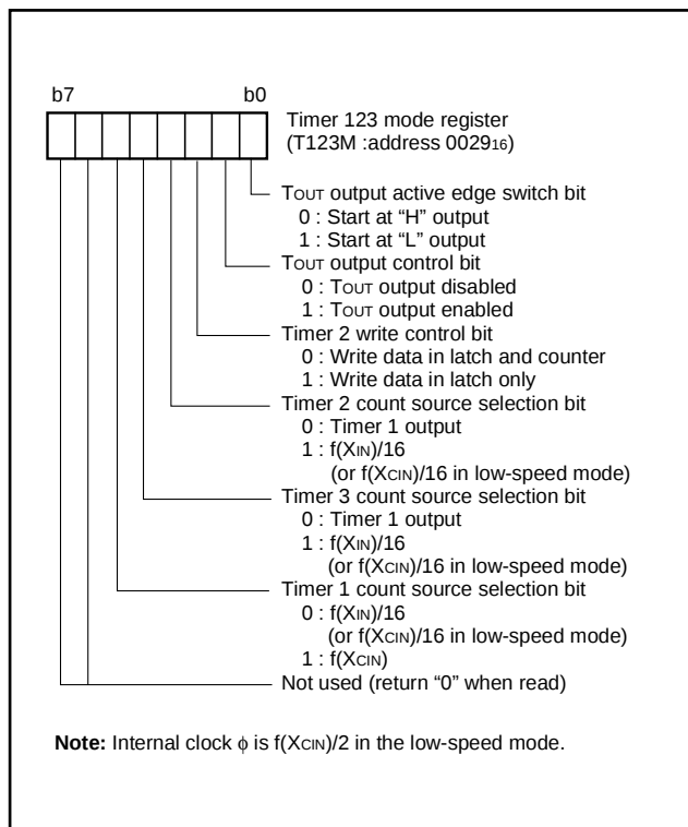
Fig. 24 Structure of timer 123 mode register
