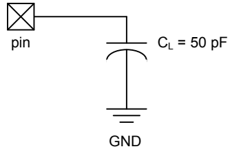
Figure 20-1. Load Conditions
