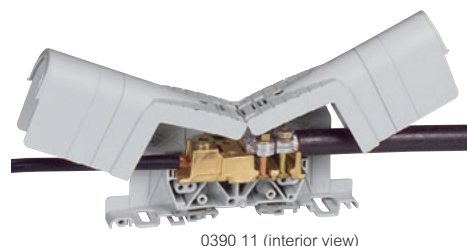
0390 11 (interior view)
