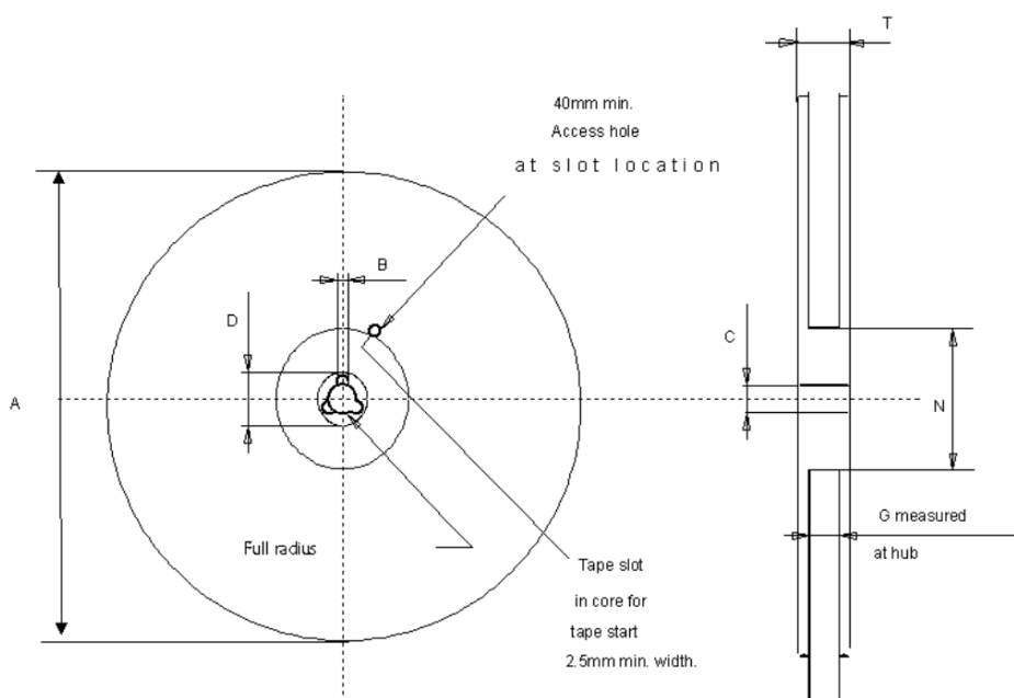
Figure 47. PowerSSO-36 reel 13"
