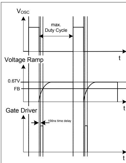
Figure 7 Light Load Conditions
