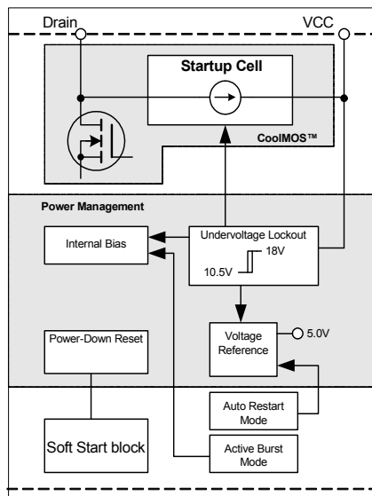
Figure 3 Power Management
