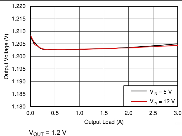
Figure 6-3. BUCK1, PSM Mode, Load Regulation
