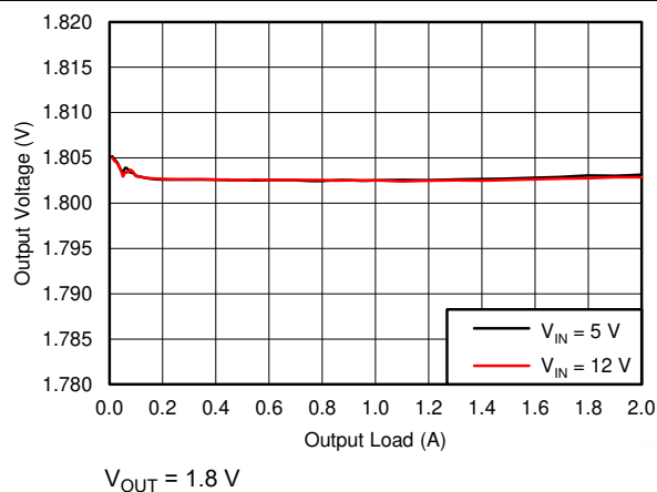
Figure 6-5. BUCK3, PSM Mode, Load Regulation
