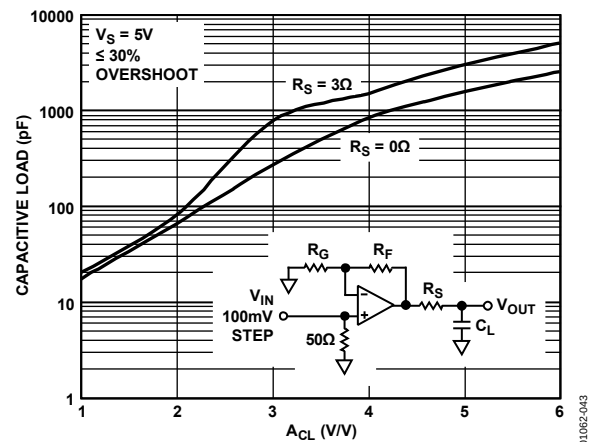
Figure 44. AD8051/AD8052 Capacitive Load Drive vs. Closed-Loop Gain
