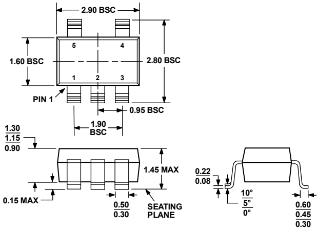
COMPLIANT TO JEDEC STANDARDS MO-178-AA Figure 54. 5-Lead Small Outline Transistor Package [SOT-23] (RJ-5)
