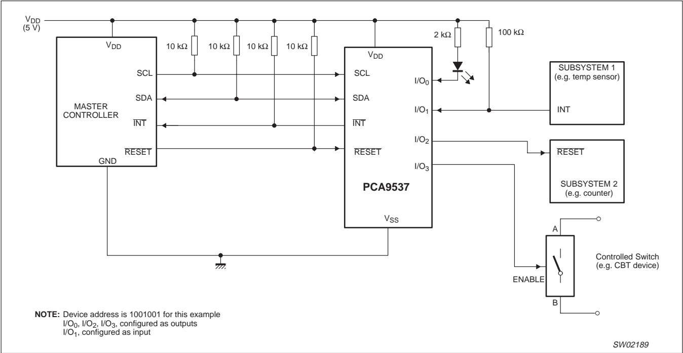
Figure 9. Typical application
