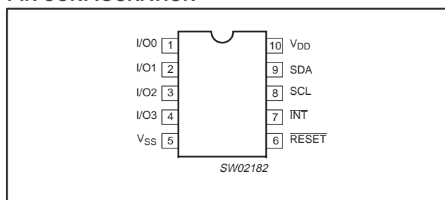
Figure 1. Pin configuration
