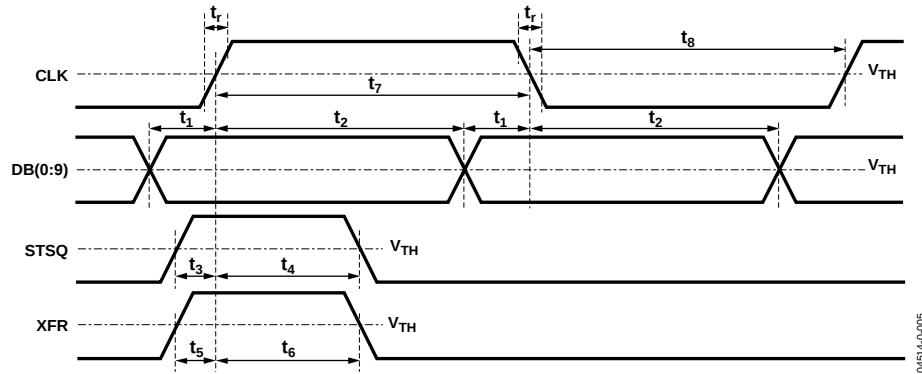
Figure 5. Input Timing
