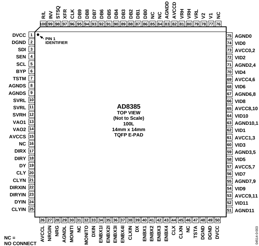
Figure 3. 100-Lead TQFP Package
