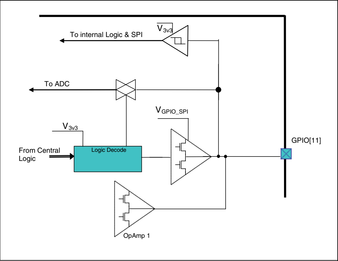
Figure 41. GPIO[11] block diagram
