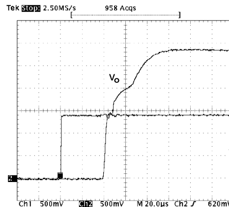
Figure 21. Startup
