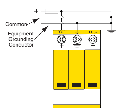
Application C One energized pole/mode 600Vdc & 1000Vdc*** systems only (Max. system discharge current (8/20 \mu s) [ I_{max} ] 25kA)
