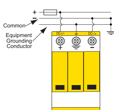
Application B One energized pole/mode 600Vdc & 1000Vdc*** systems only
