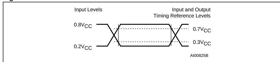
Figure 19. AC measurement I/O waveform
