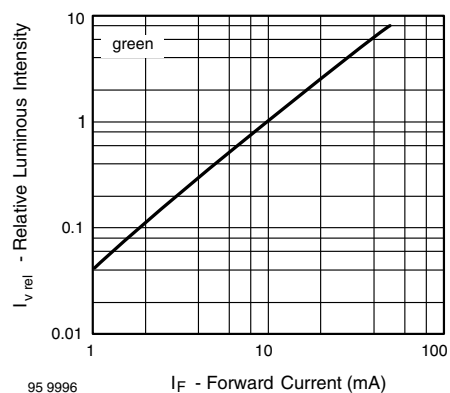
Fig. 22 - Relative Luminous Intensity vs. Forward Current
