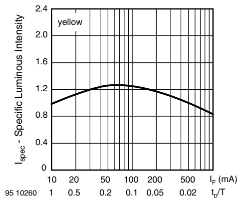
Fig. 16 - Specific Luminous Intensity vs. Forward Current/Duty Cycle
