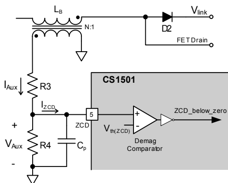
Figure 18. ZCD Input Pin Model
