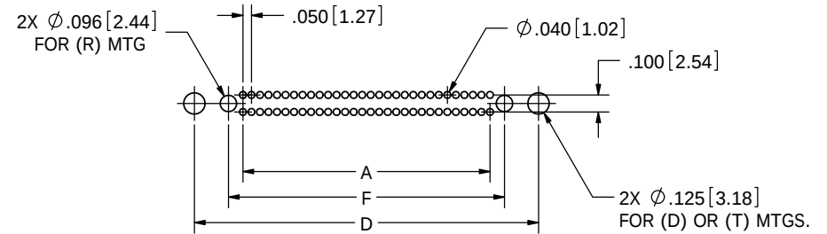
PCB LAYOUT, CONNECTOR SIDE
