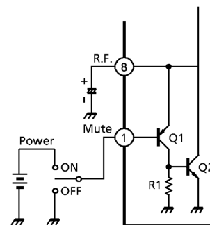
Fig.5 Mute circuit
