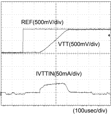
Fig.10 Soft start
