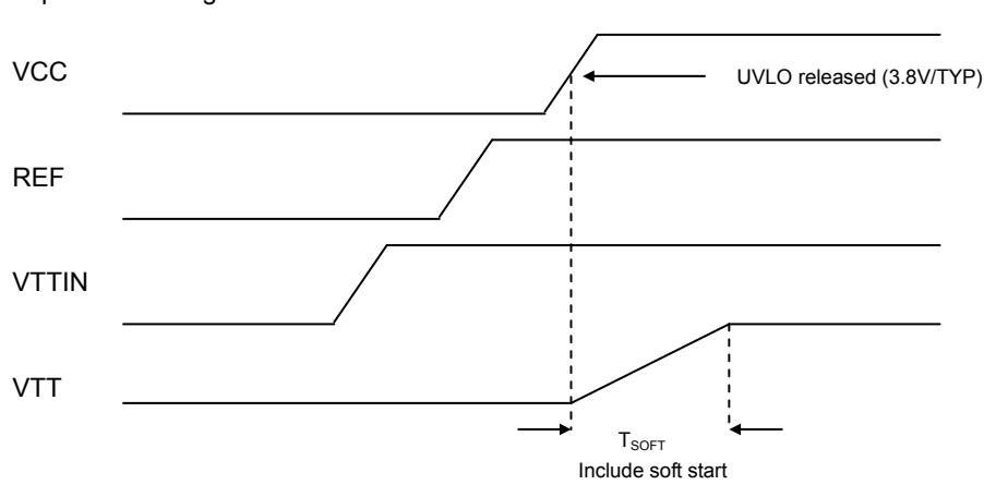
(b) when input VCC voltage
