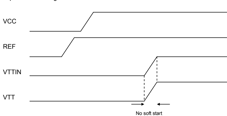
(c) when input VTTIN voltage
