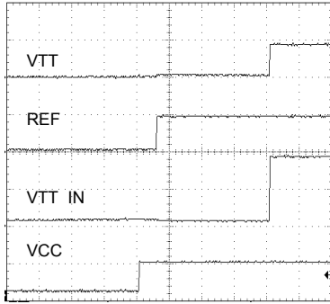
Fig.6 Input Sequence 2
