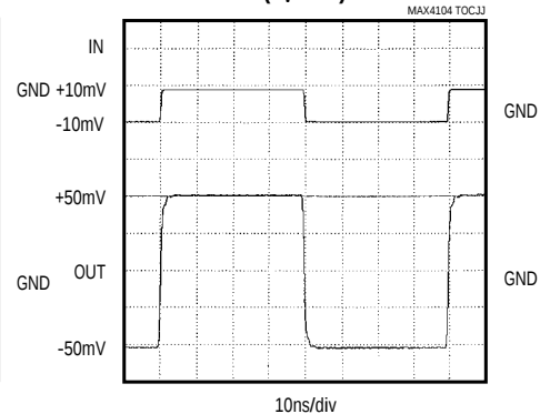
MAX4105 SMALL-SIGNAL PULSE RESPONSE ( A_V = +5 )
