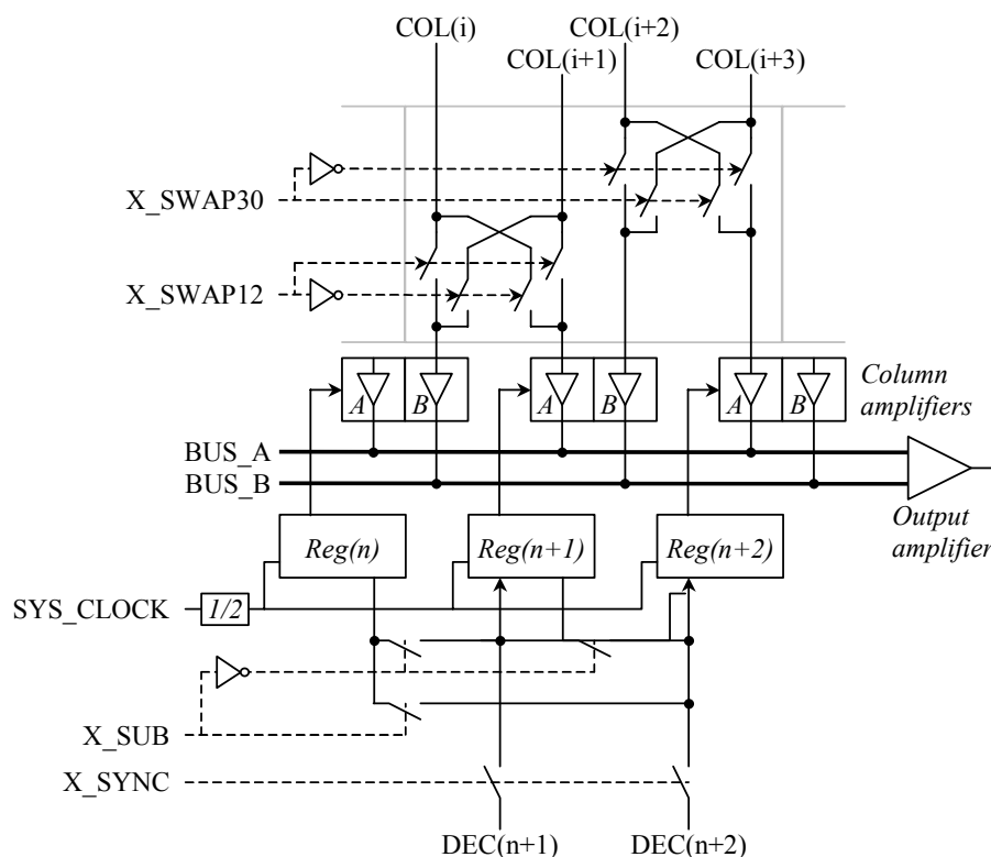
Figure 8: Column structure
